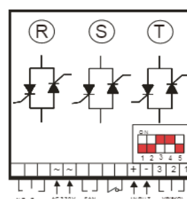
3. Input Signal manual + 4-20mA
